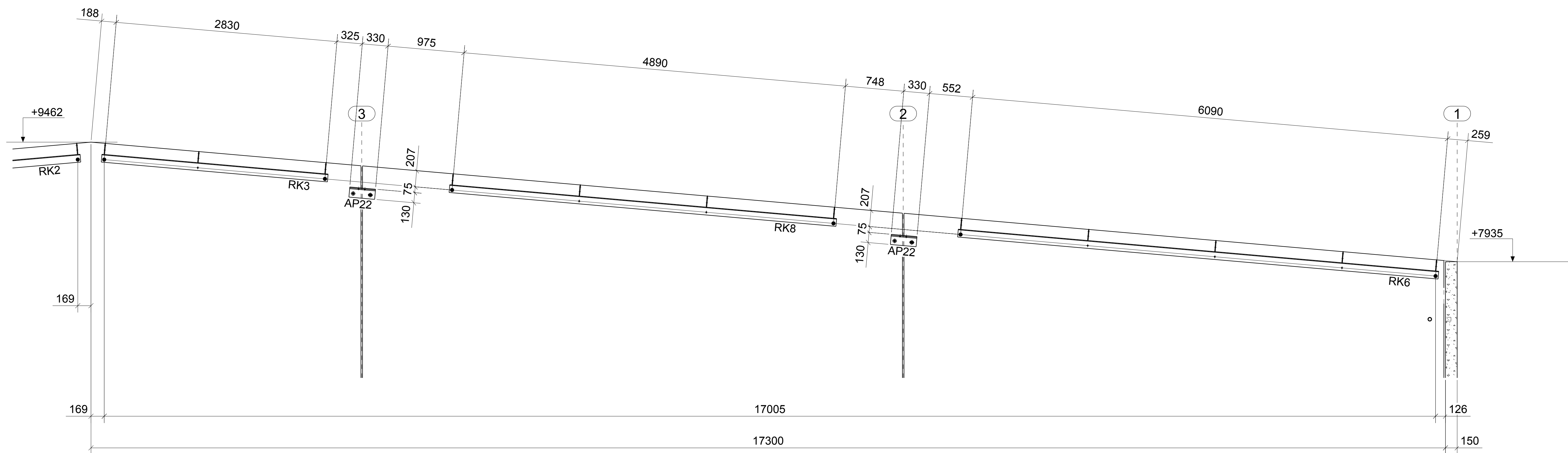
PART ELEVATION INSIDE PANELS GRID A
