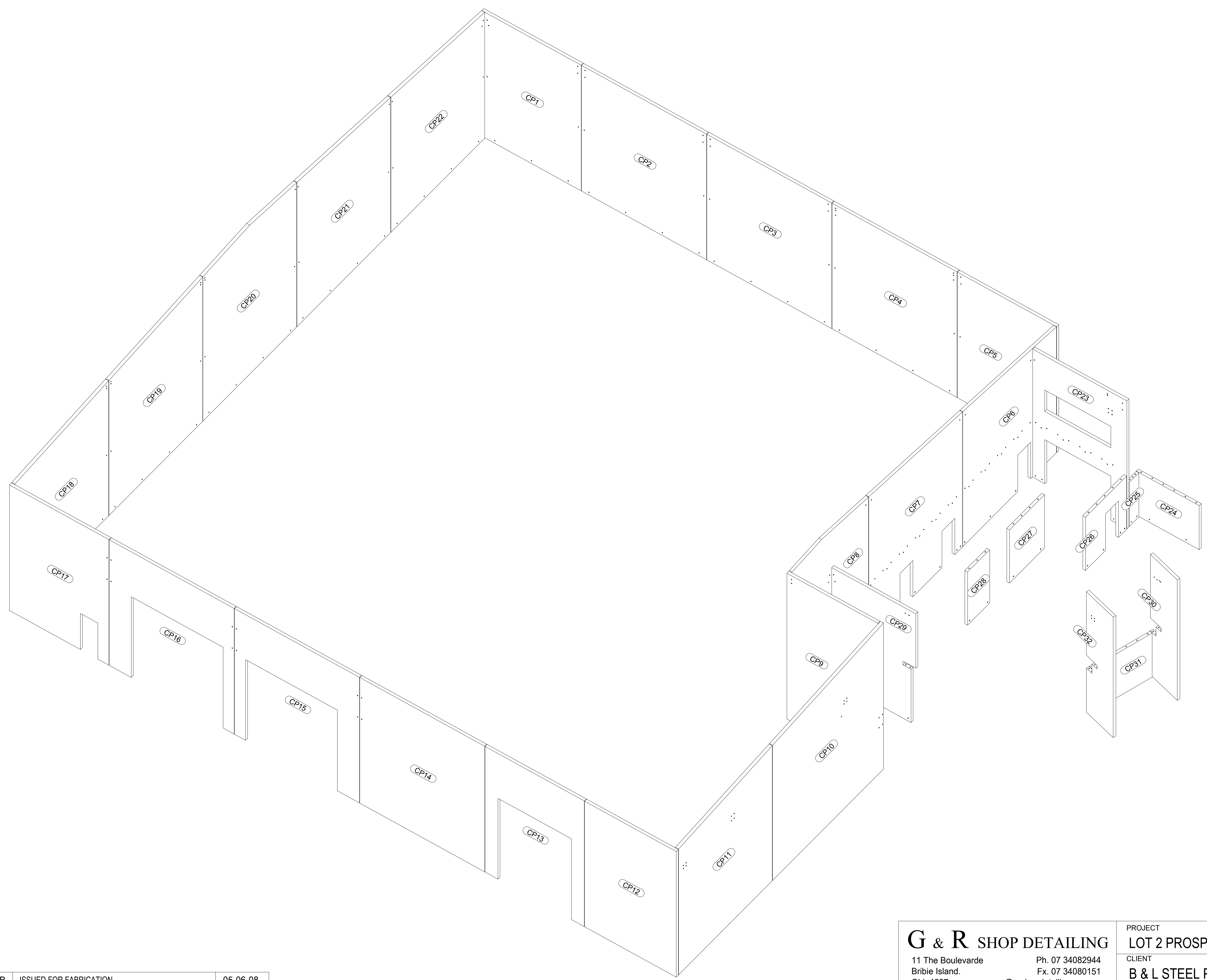
TILT PANELS PERSPECTIVE VIEW
